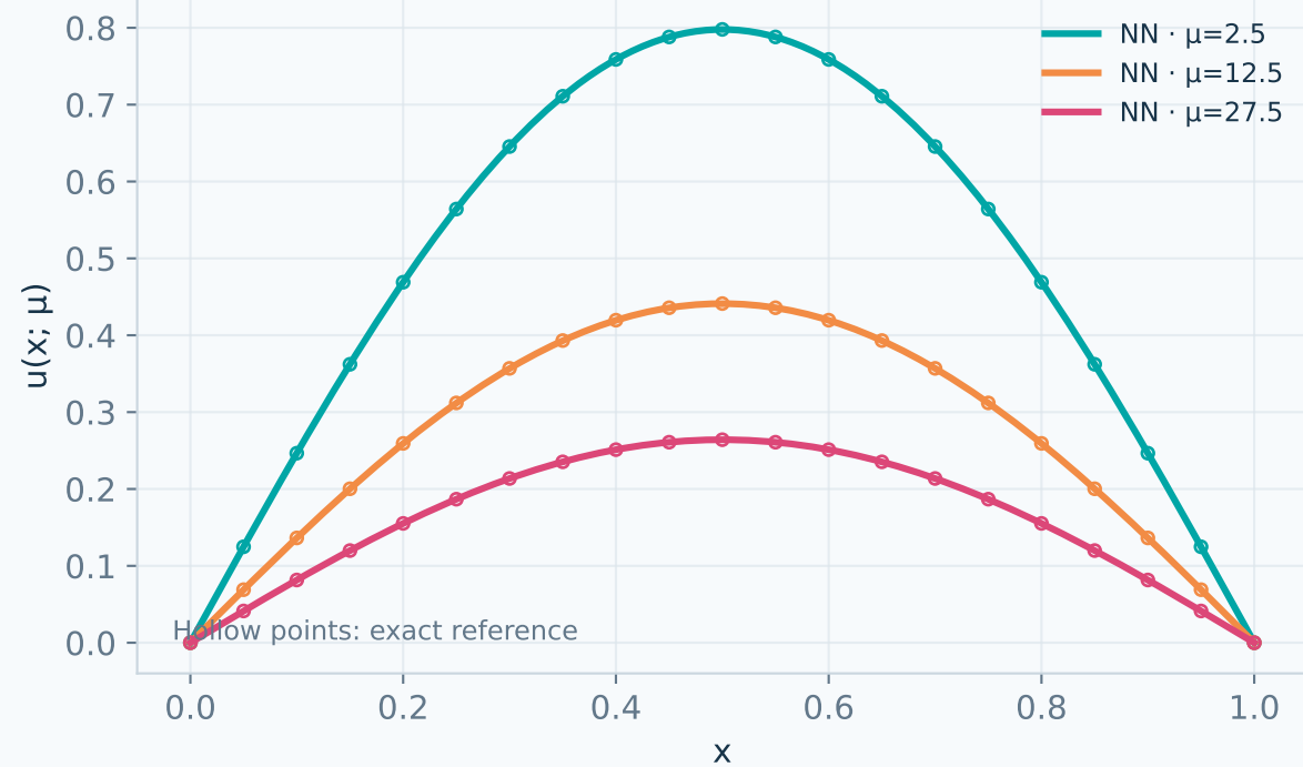
New parameter queries after training
